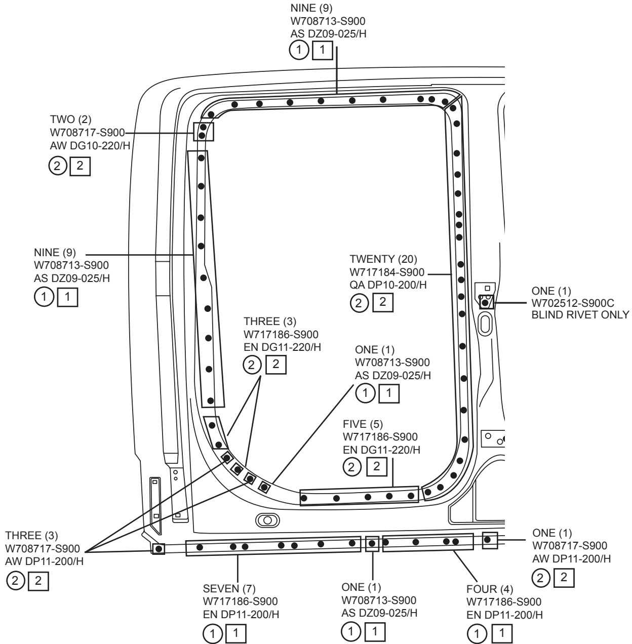
FIGURE 2 REAR DOOR OPENING
